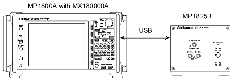
Figure 2.5.2-1 Connecting MP1800A
